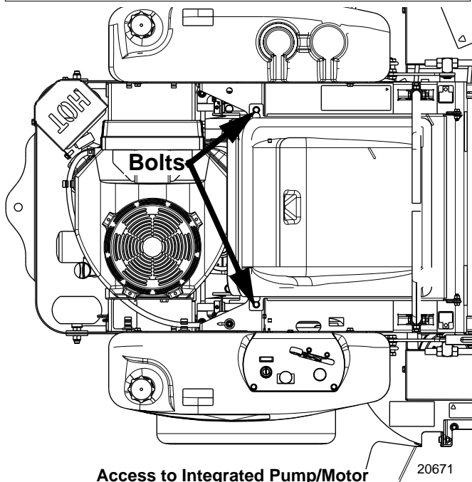
Access to Integrated Pump/Motor Figure 4-4
