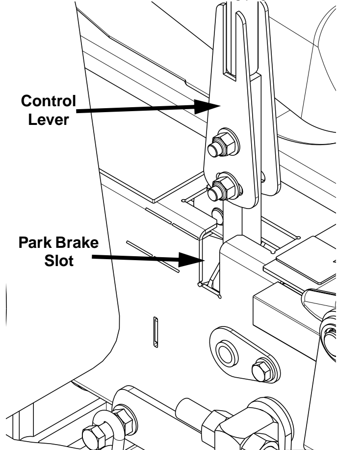
Control Lever In Neutral Position Figure 3-1
