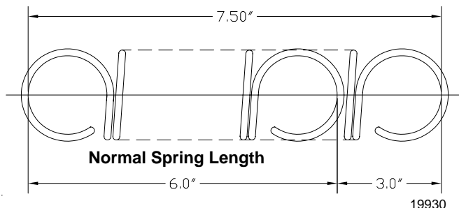
Spring Tension Figure 3-7
