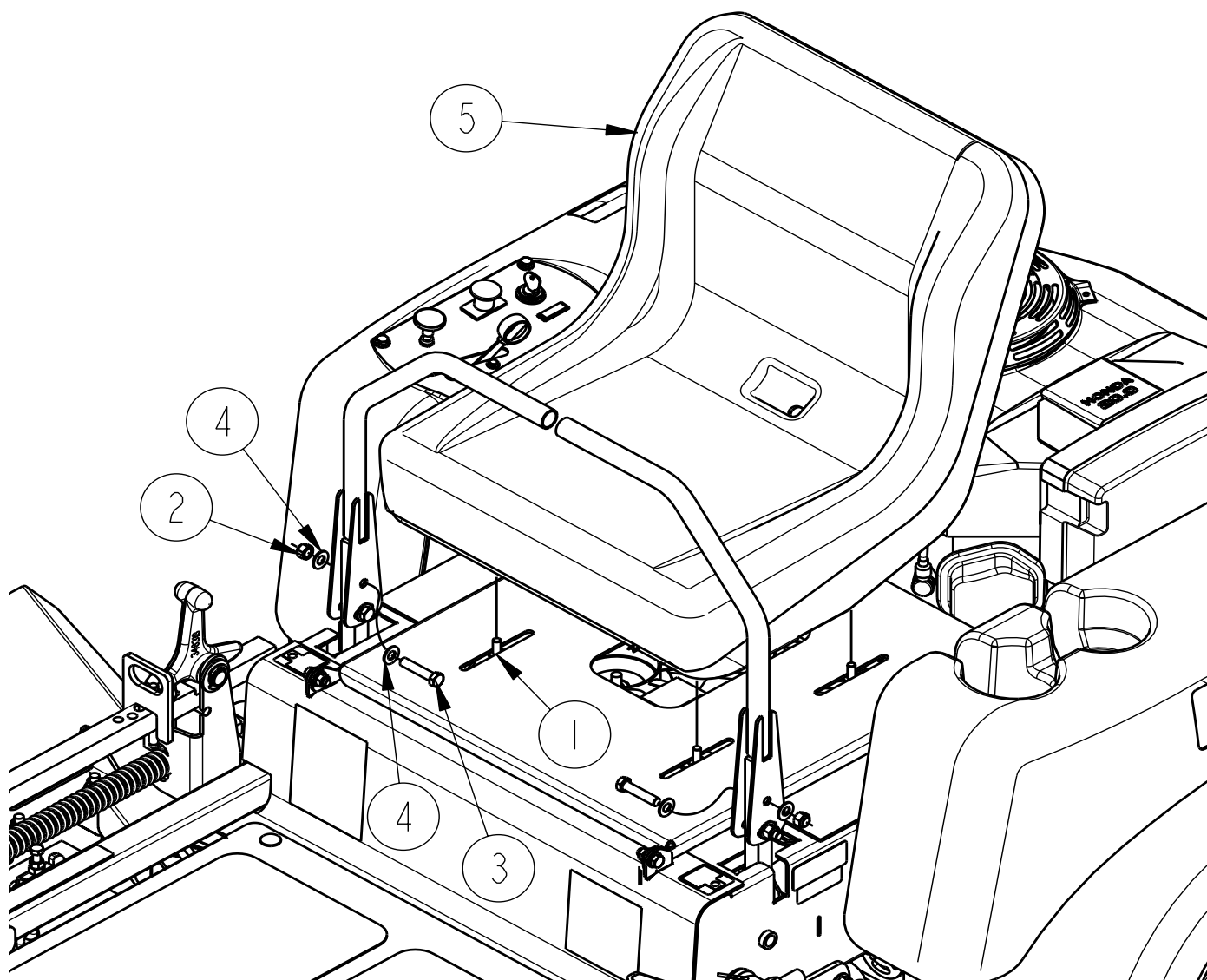
Control Lever & Seat Assembly Figure 1-1
