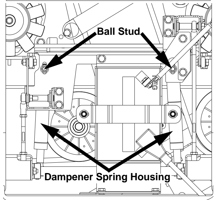
Steering Dampener Figure 3-3
