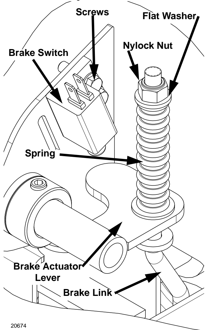
Brake Adjustments Figure 3-5
