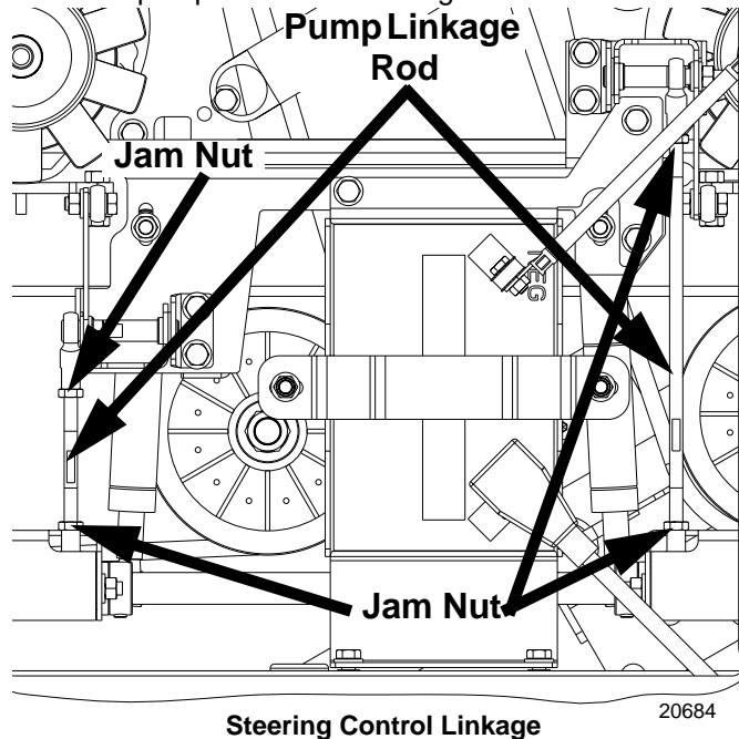
Steering Control Linkage Figure 3-2
